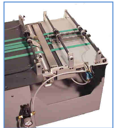
Optional divert gate for wrong products. Divert gate activated by vision system.
