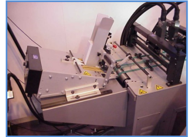
KR496F Friction feeder for plastic cards
